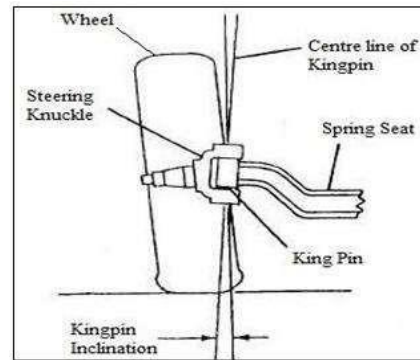
Components of Front axle beam
