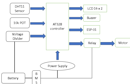
Figure 1: Block Diagram
