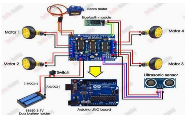
Figure 4: Overall circuit diagram used for the project work
