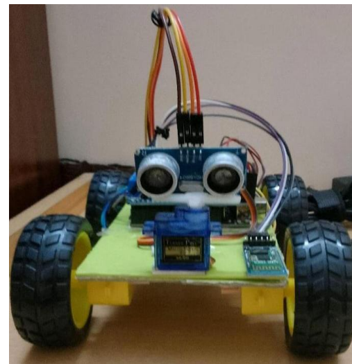
Figure 7: Model of the robotic vehicle developed - 2
